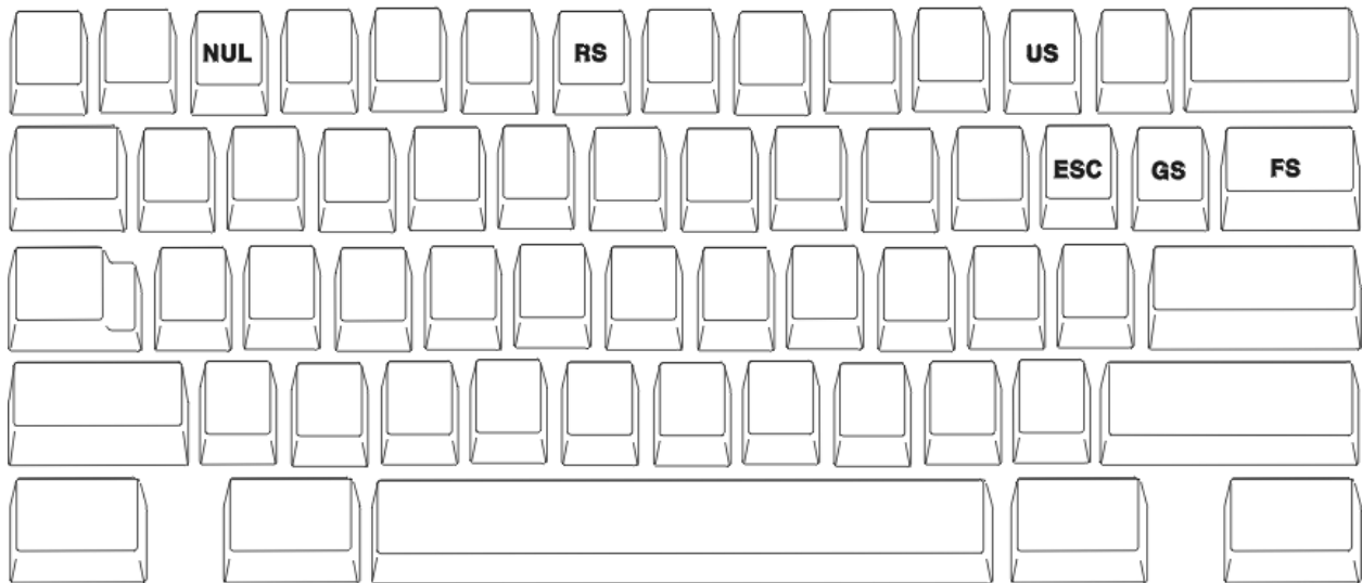
Figure 6. Common Control Code of Keyboard Core Segment for Non-Japanese Keyboard on page 4
