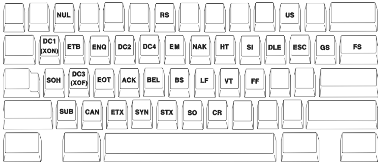
Figure 8. Control-Code Map of Keyboard Core Segment for U.S. Enhanced Keyboard on page 4
