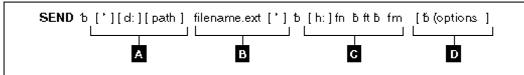
Figure 1. VM/CMS SEND Command Syntax
