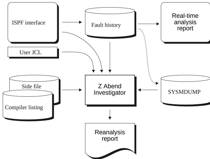
Figure 5. Reanalysis
