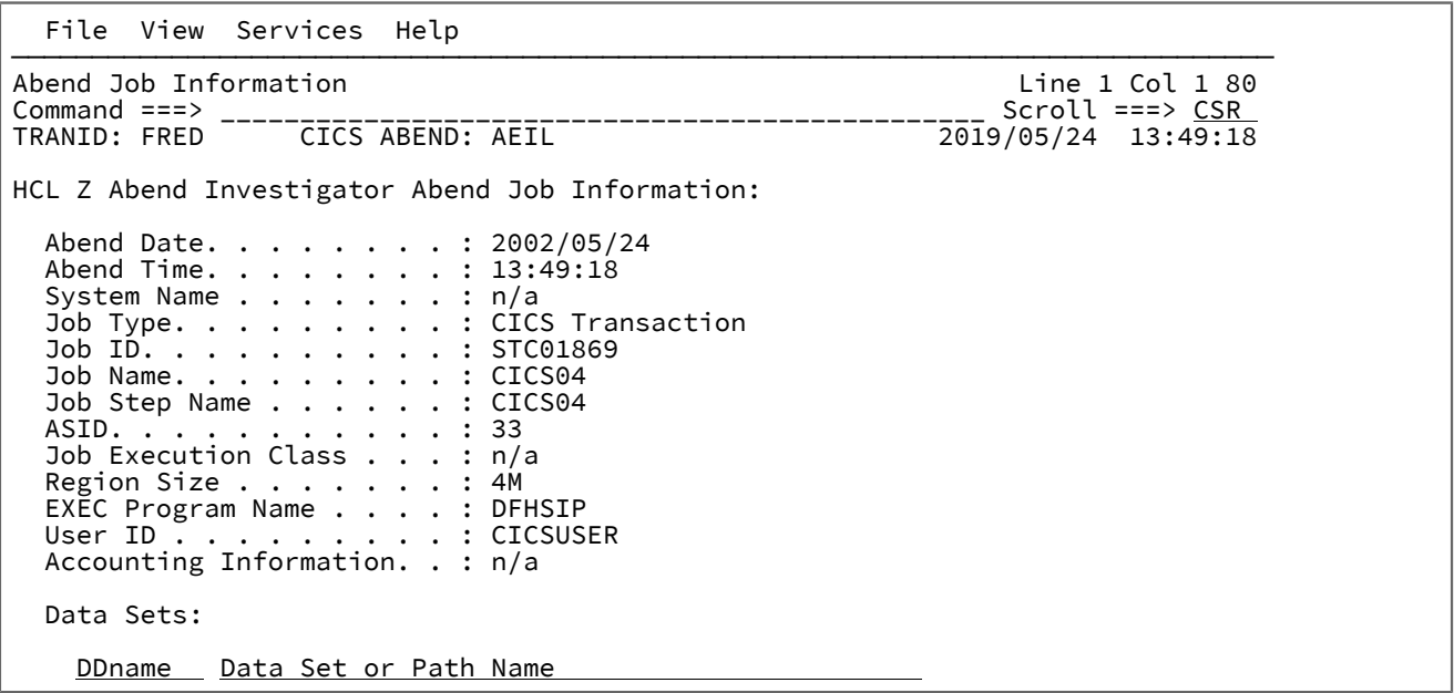
Figure 129. Sample Abend Job Information display
