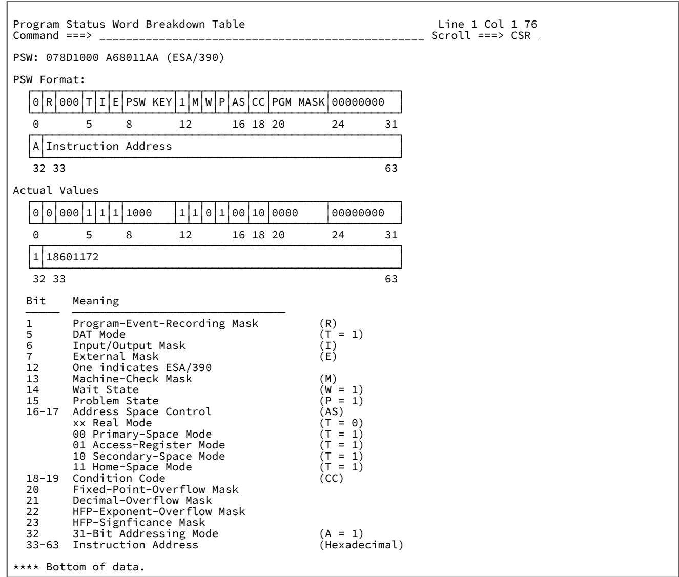
Figure 148. Sample Program Status Word Breakdown Table display
