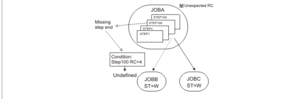
Figure 171. Step dependency status evaluation if no step-end event is received for Step100 and JOBA ends in error
