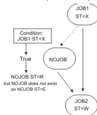
Figure 173. An example of how to set to W the status of an operation with predecessors in X status
