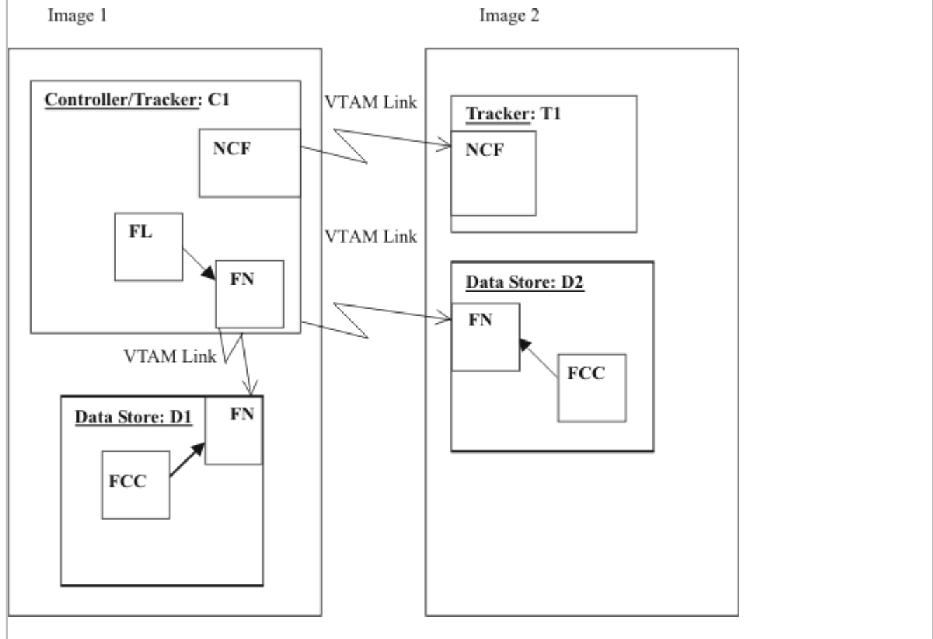
Figure 5. Controller and tracker in same address space with tracker connected through SNA
