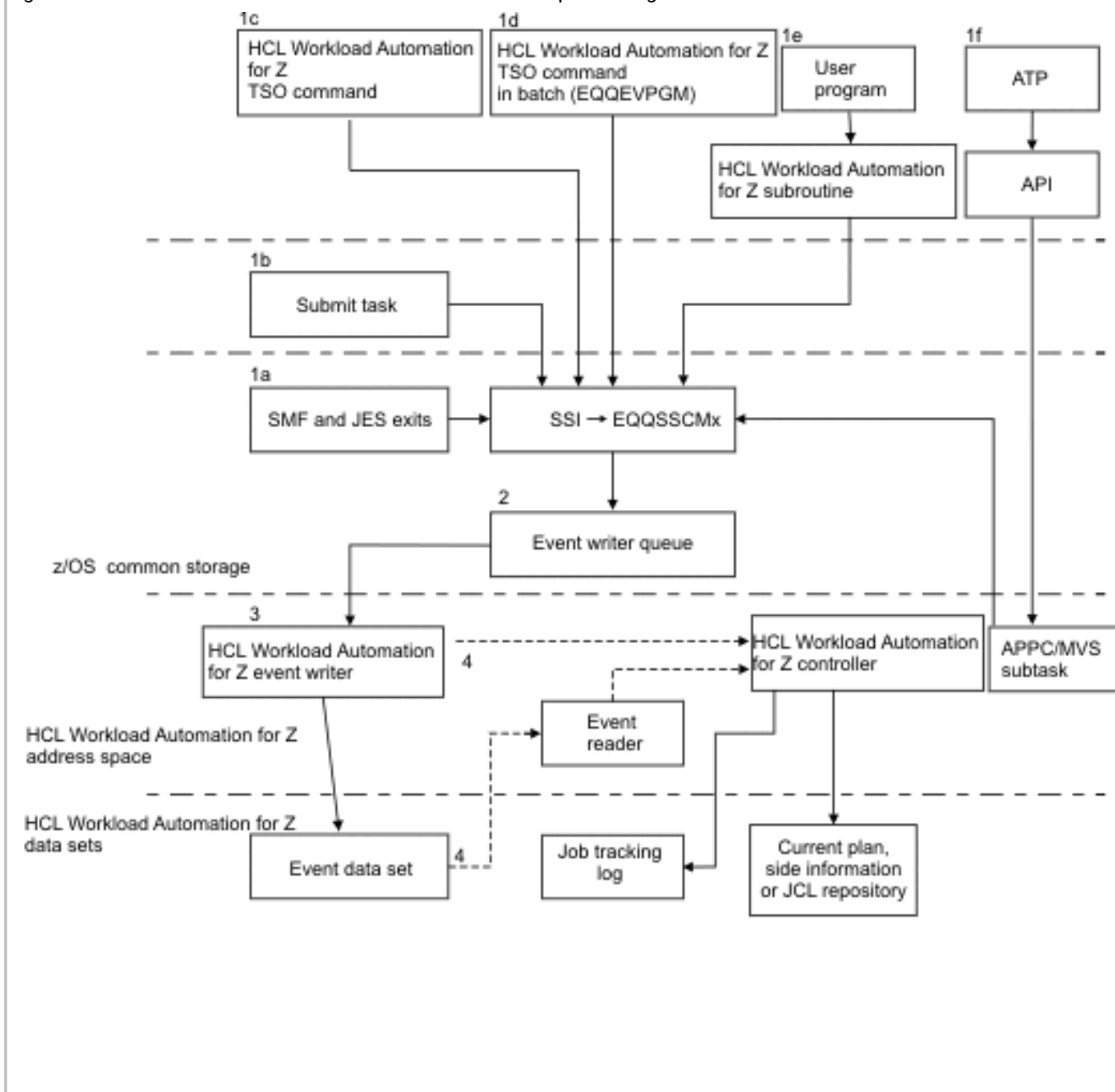
Figure 6. HCL Workload Automation for Z event creation and processing
