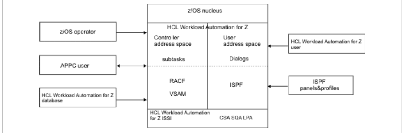
Figure 1. HCL Workload Automation for Z dialog structure
