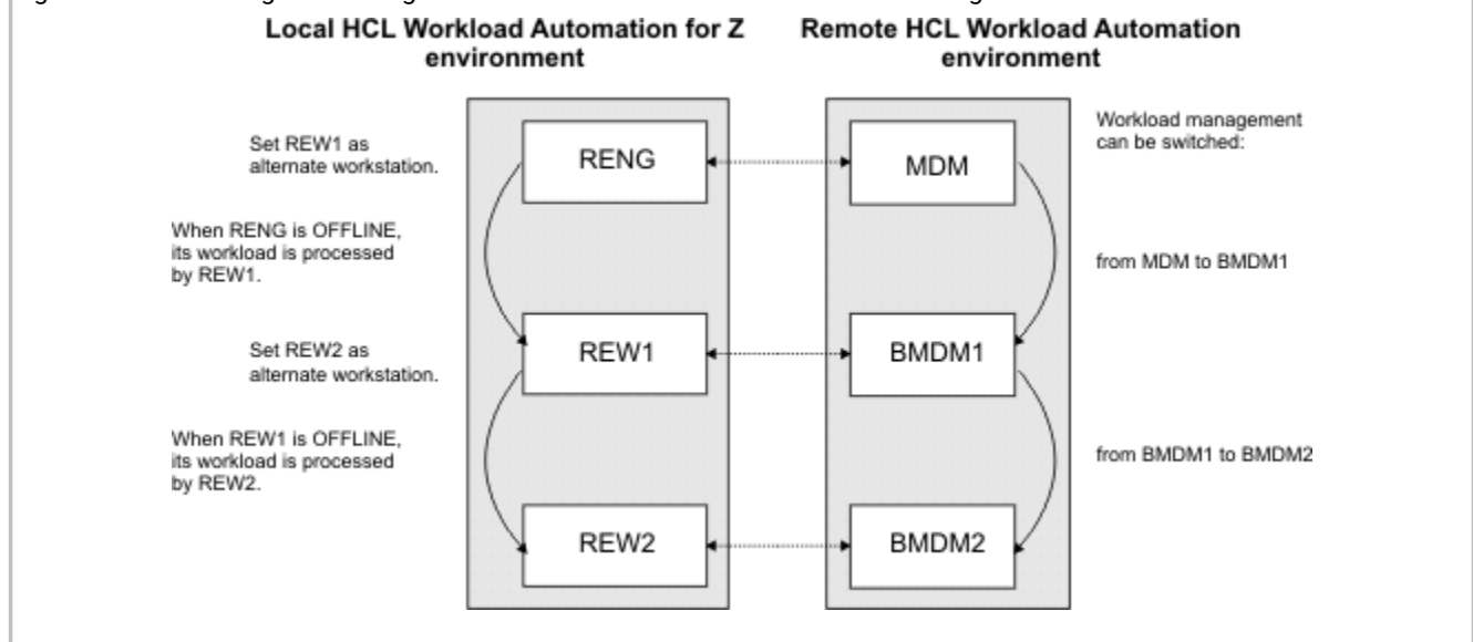
Figure 199. Cascading remote engine workstation definitions for the switch management scenario
