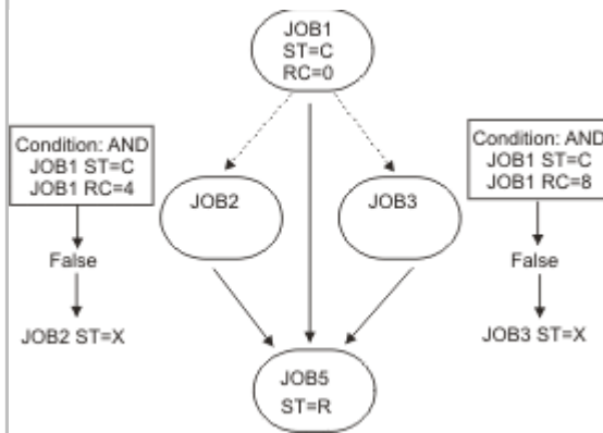
Figure 159. Successors status evaluation if JOB1 ends with status C and return code 0
