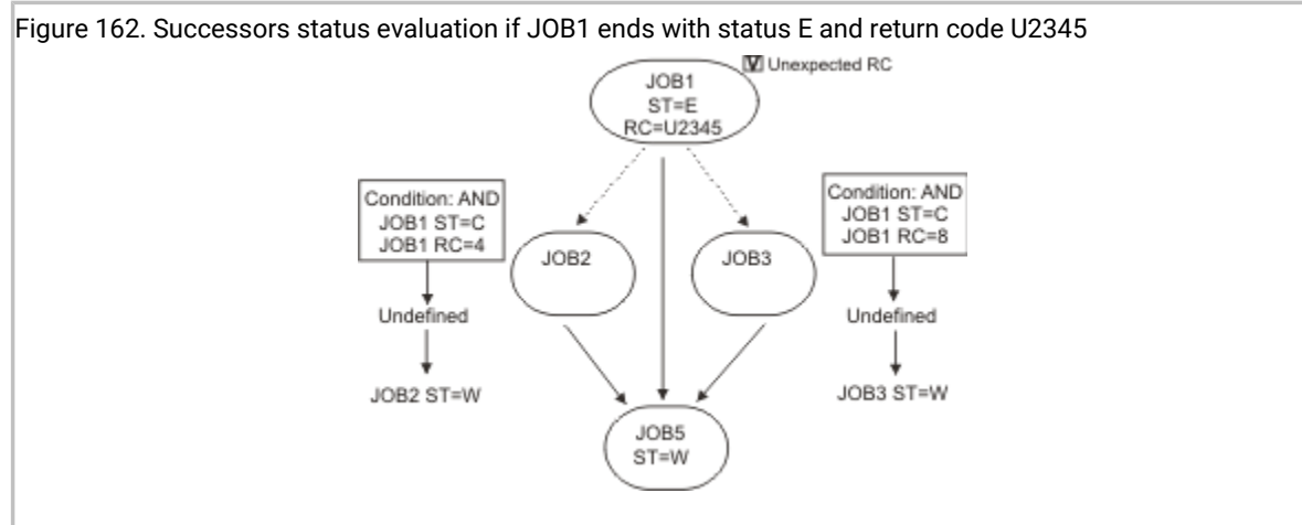
Figure 162: Successors status evaluation if JOB1 ends with status E and return code U2345 on page 408
