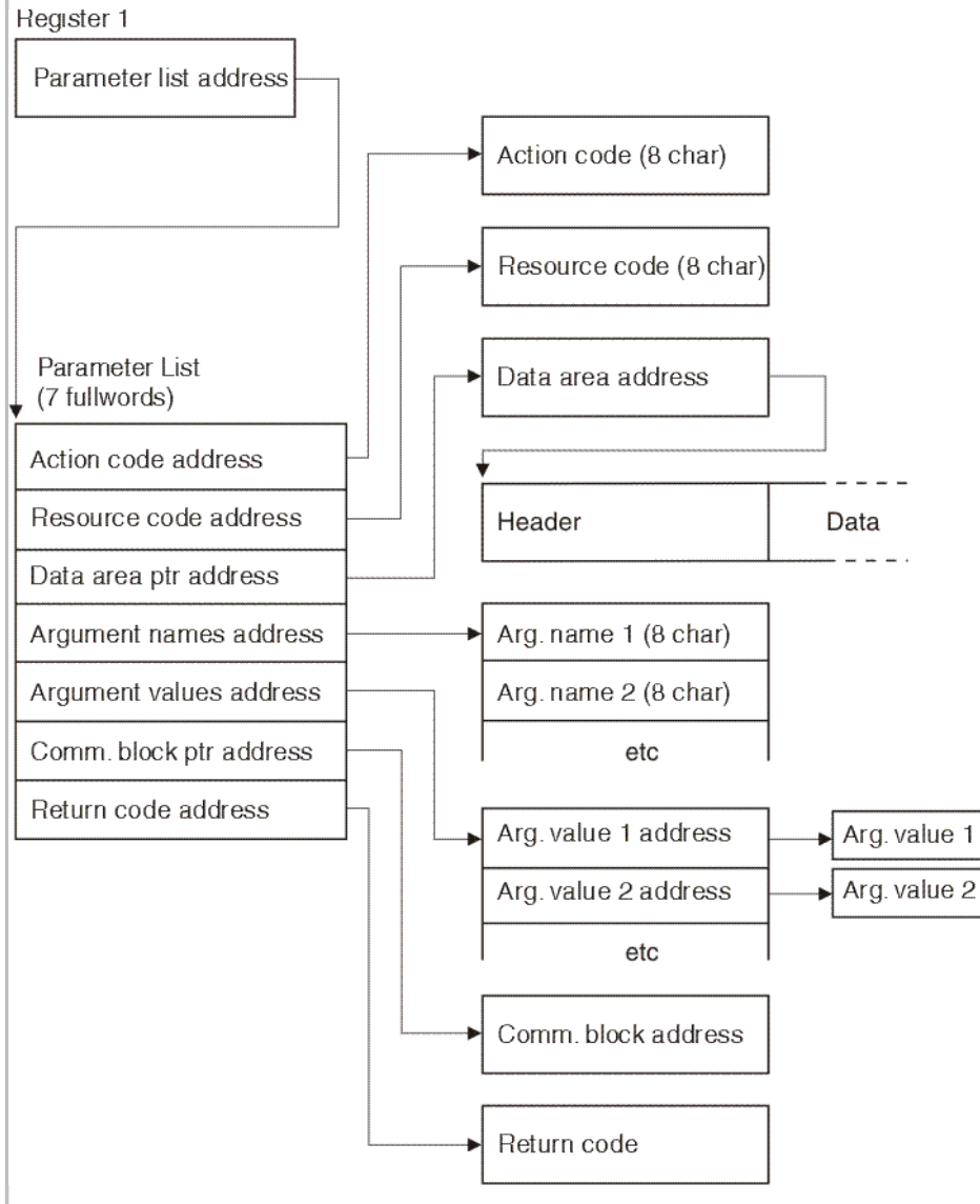
Figure 1. Program interface parameters
