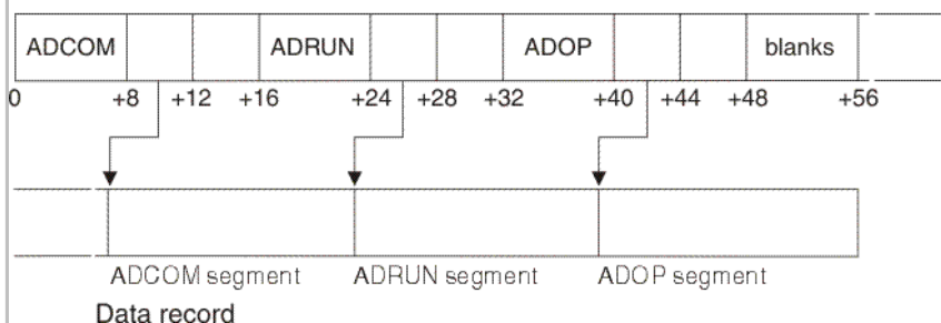
Figure 3. Program interface data area example
