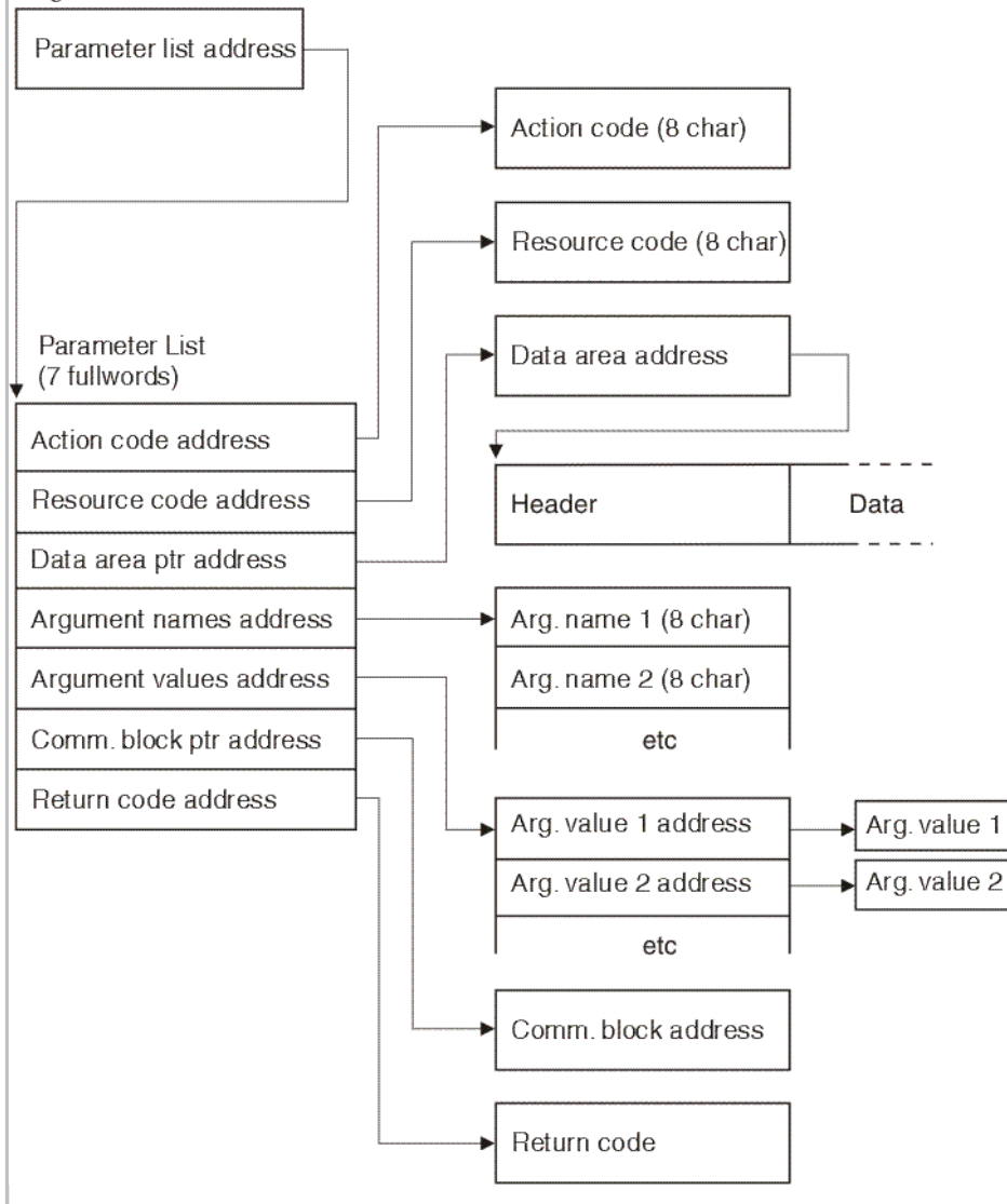
Figure 1. Program interface parameters
