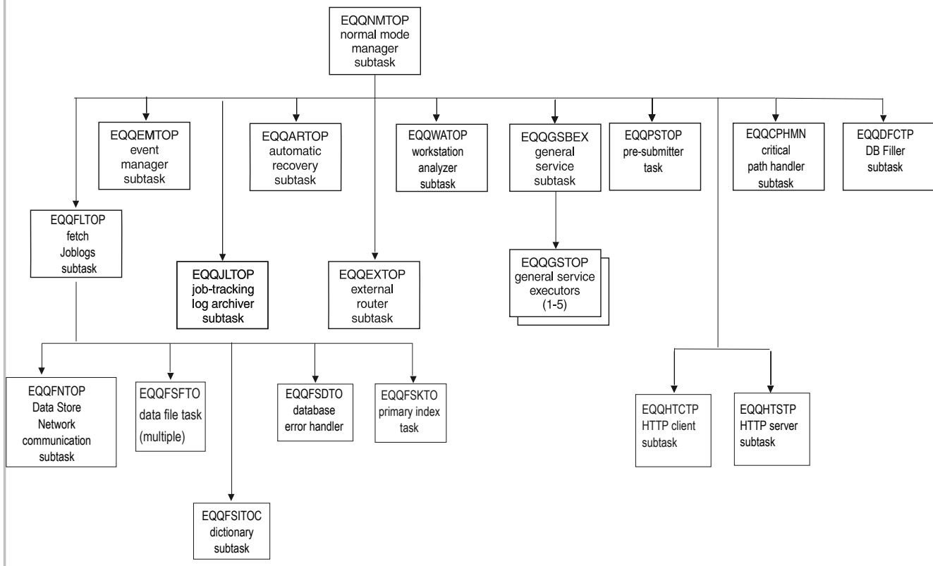
Figure 3. Z controller subtasks
