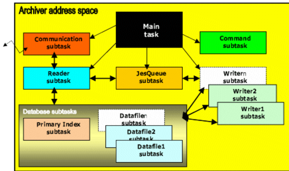
Figure 5. HCL Workload Automation for Z data store address space structure
