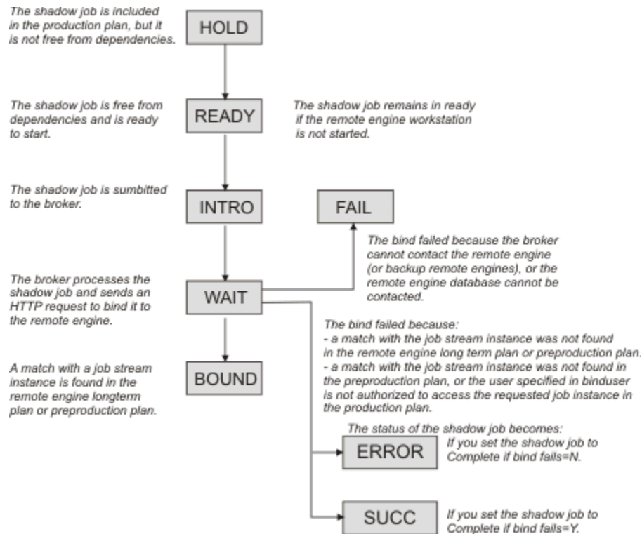
Figure 38. Shadow job status transition until the bind is established
