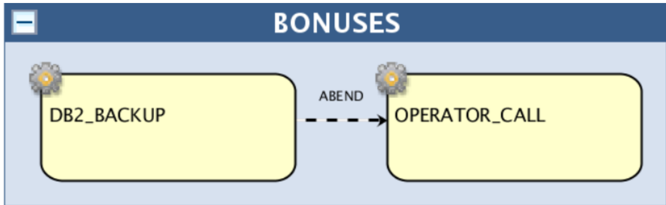
Figure 33. ABEND status conditional dependency
