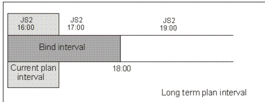
Figure 42. The instance to be bound exists but it is not yet included in the CP
