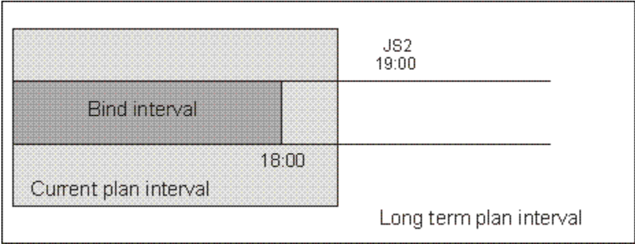
Figure 41. The scheduled time of the shadow job is included in the CP but no instance to bind exists
