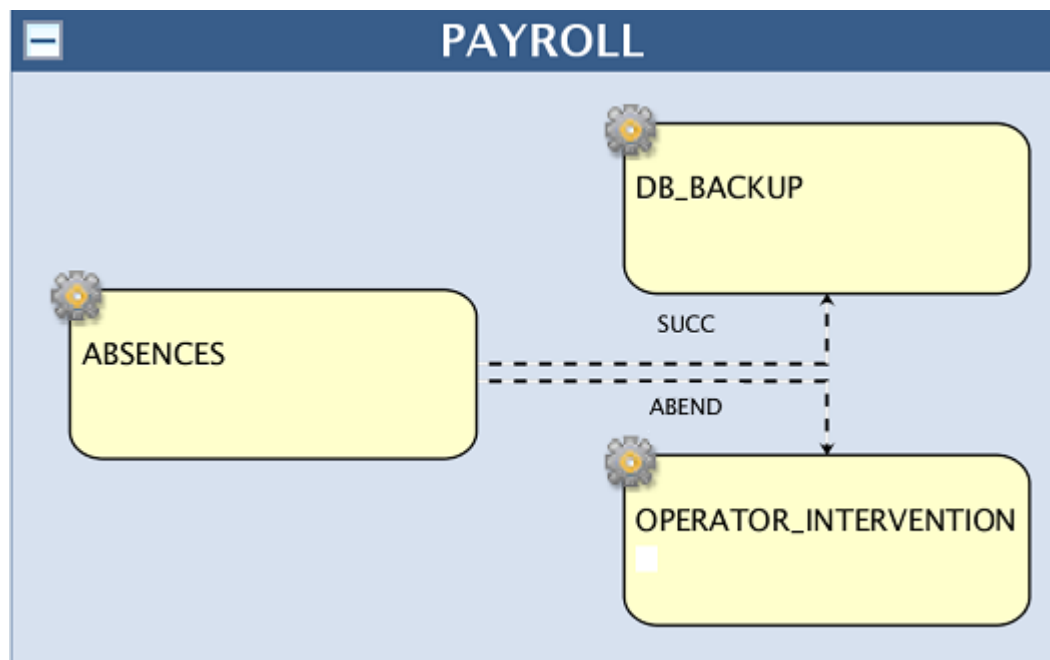
Figure 29. Two different conditional dependencies on SUCC and ABEND statuses on the ABSENCES job
