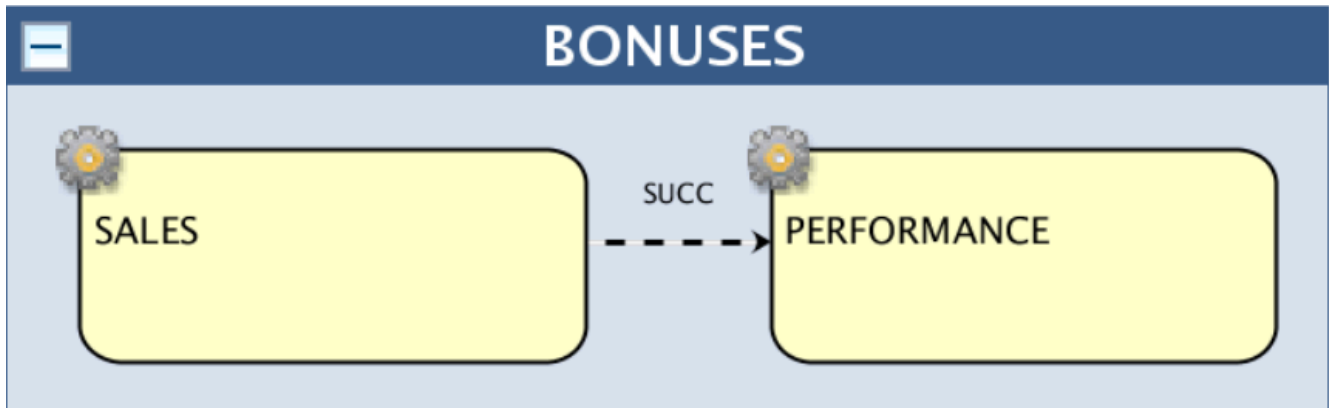
Figure 32. Status conditional dependency on a job with recovery stop setting
