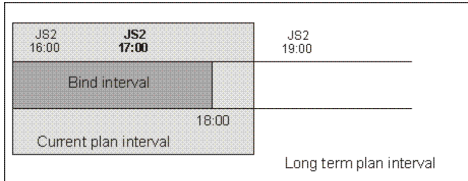
Figure 39. Instance to be bound if the shadow job scheduled time is included in the CP interval
