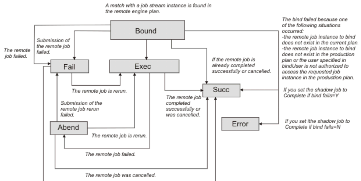
Figure 44. Shadow job status transition chain after the bind was established
