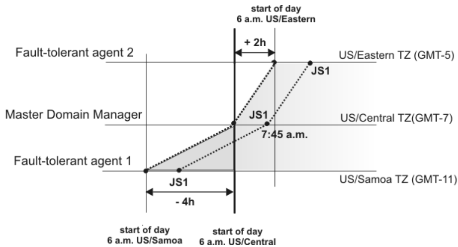
Figure 25. Example when start of day conversion is not applied
