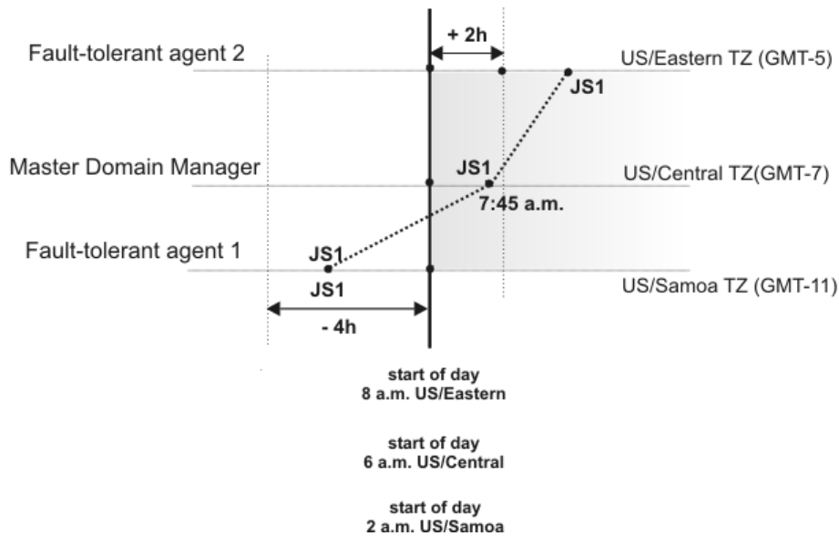
Figure 26. Example when start of day conversion is applied
