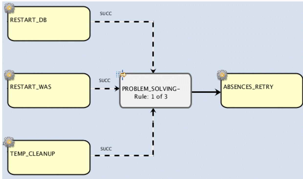
Figure 31. A join dependency containing three dependencies on SUCC status
