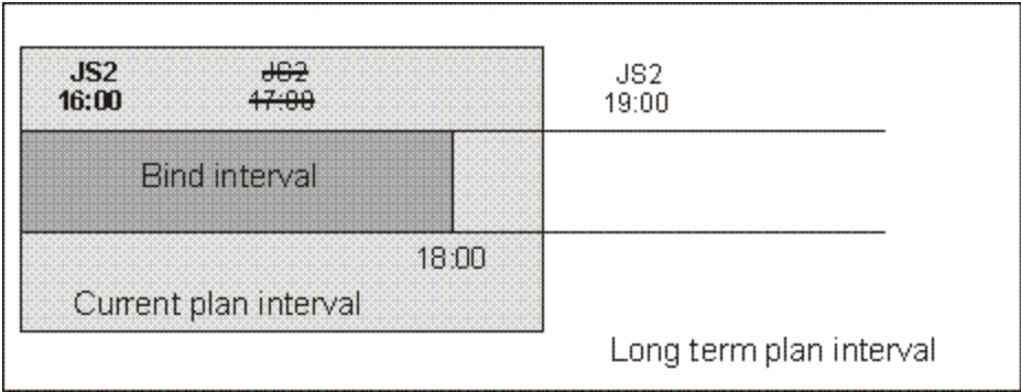
Figure 40. Instance to be bound if the instance that most closely precedes the shadow job scheduled time exists in the LTP but was canceled from the CP
