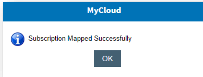
Figure 174 - Confirmation Message
