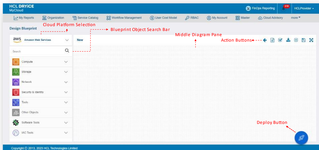
Figure 386 - Design Blueprint
