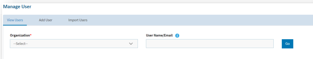
Figure 12 – Manage User
