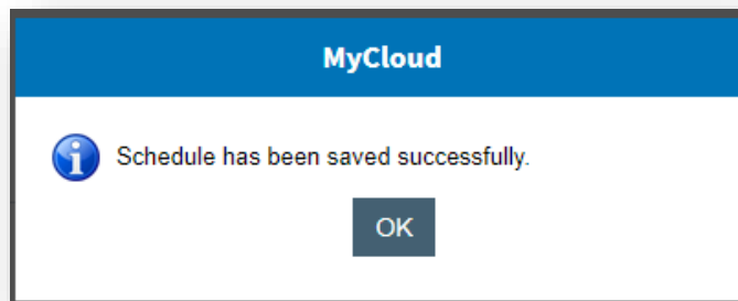
Figure 212 - Success Schedule
