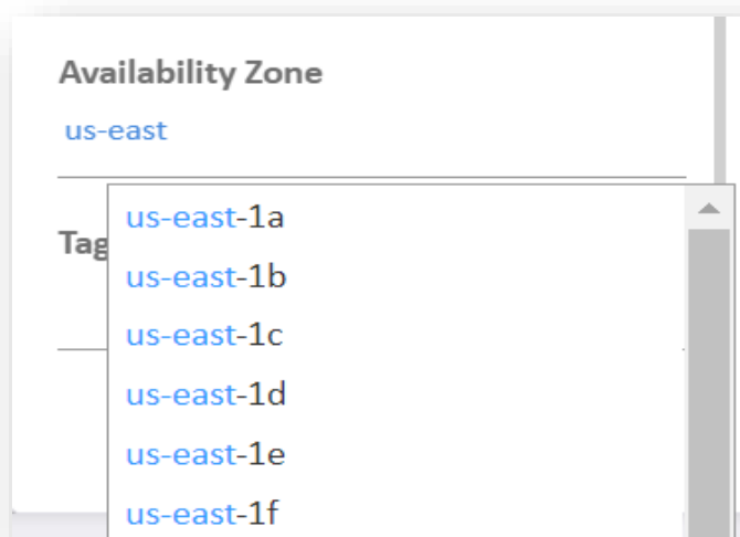
Figure 398 – Zone Mapping
