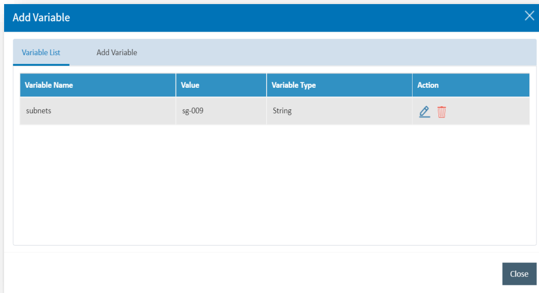
Figure 419 – Delete Variable
