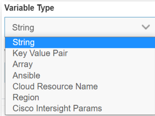
Figure 407 – Variable Type
