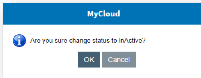
Figure 306 – Confirmation Message
