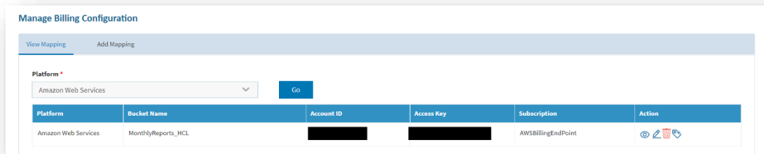
Figure 149 – View Mapping
