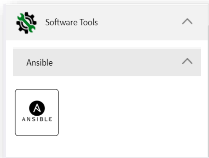
Figure 448 - Ansible Object
