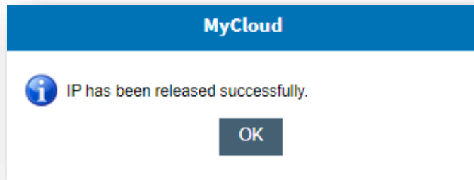
Figure 163 - Success Message
