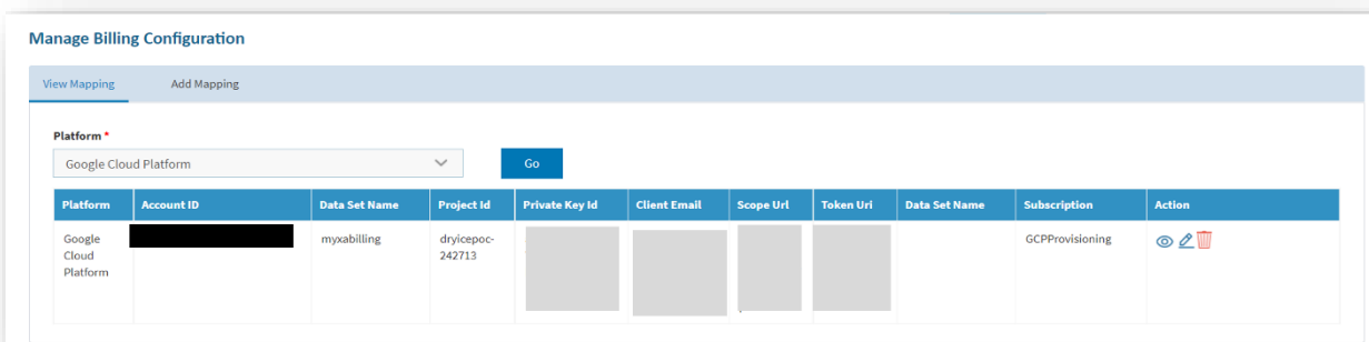
Figure 152 - Delete Mapping
