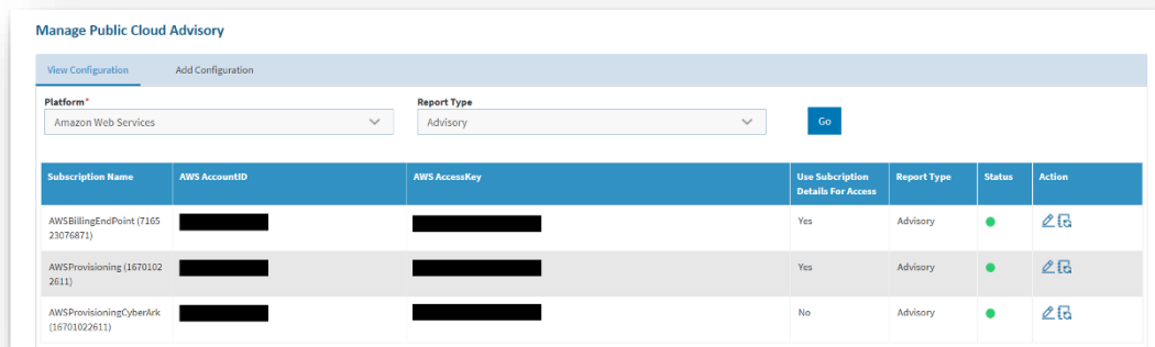
Figure 172 - Edit Configuration
