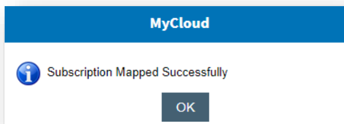
Figure 171 – Confirmation Message
