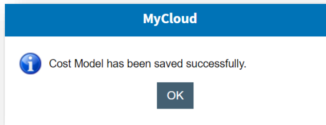
Figure 63 – Confirmation Message
