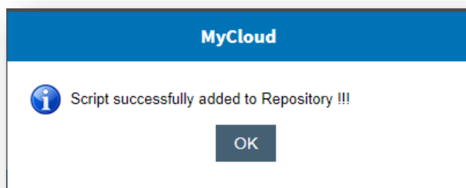
Figure 196 - Confirmation Message
