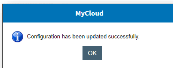
Figure 340 - Success Message
