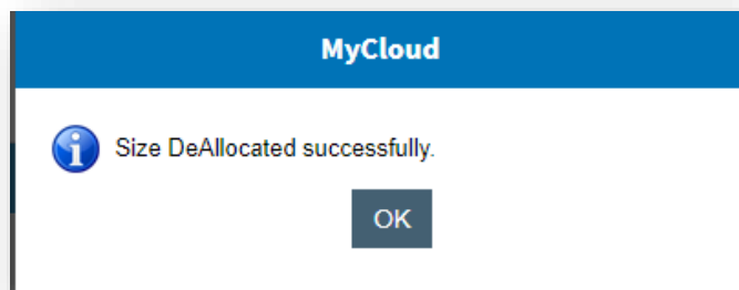
Figure 372 – Success Message
