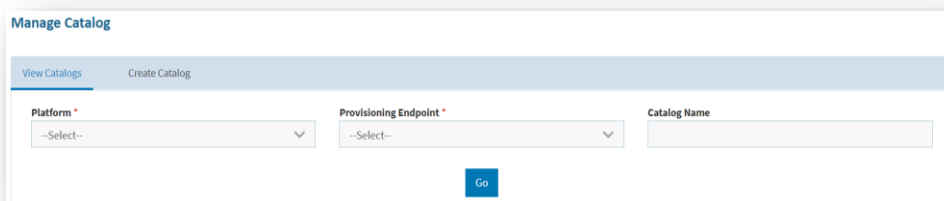
Figure 477 – Manage Catalog
