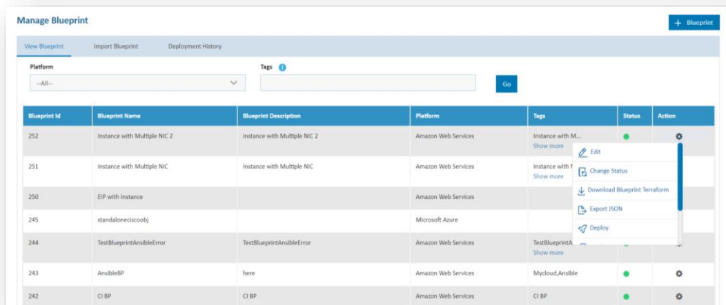
Figure 426 - View Blueprint
