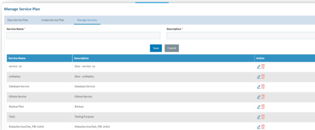
Figure 52 - Manage Services
