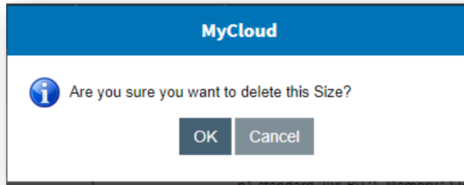
Figure 382 - Confirmation Message
