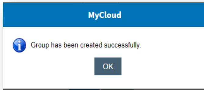
Figure 38 - Success Message
