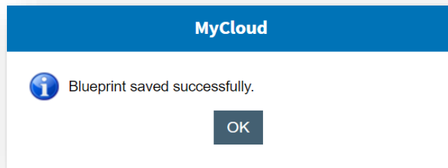
Figure 405 - Success Message
