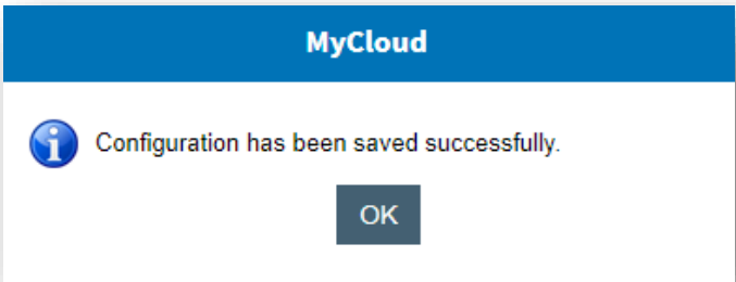
Figure 346 - Success Message
