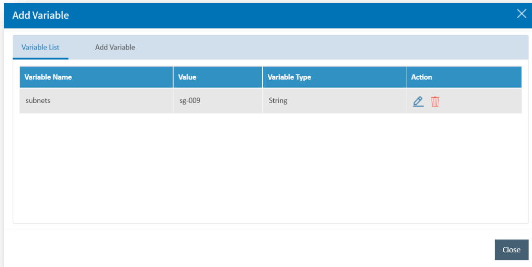
Figure 418 – Edit Variable
