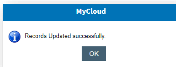
Figure 181 – Success Message
