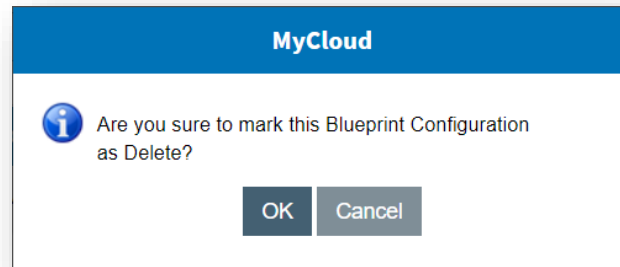
Figure 443 - Confirmation Message
