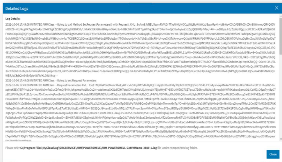
Figure 495 – Detailed Logs
