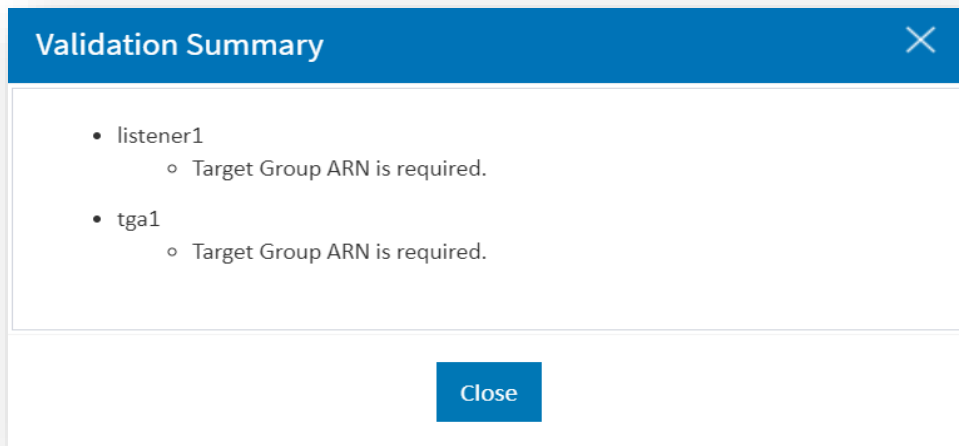
Figure 421 – Validation Summary
