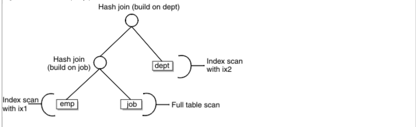
Figure 63. Possible query plan with directives
