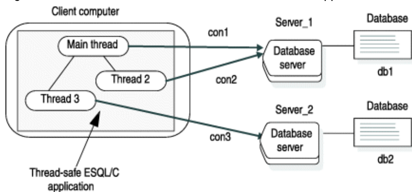
Figure 78. Concurrent connections in a thread-safe ESQL/C application
