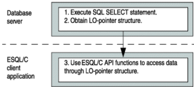
Figure 43. Transferring smart- large-object data from database server to client application
