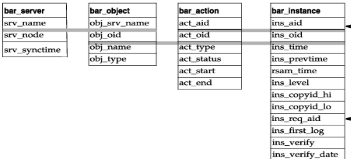
Figure 22. ON-Bar catalog map on Informix®
