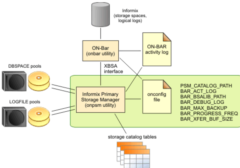
Figure 28. Components of Informix® Primary Storage Manager
