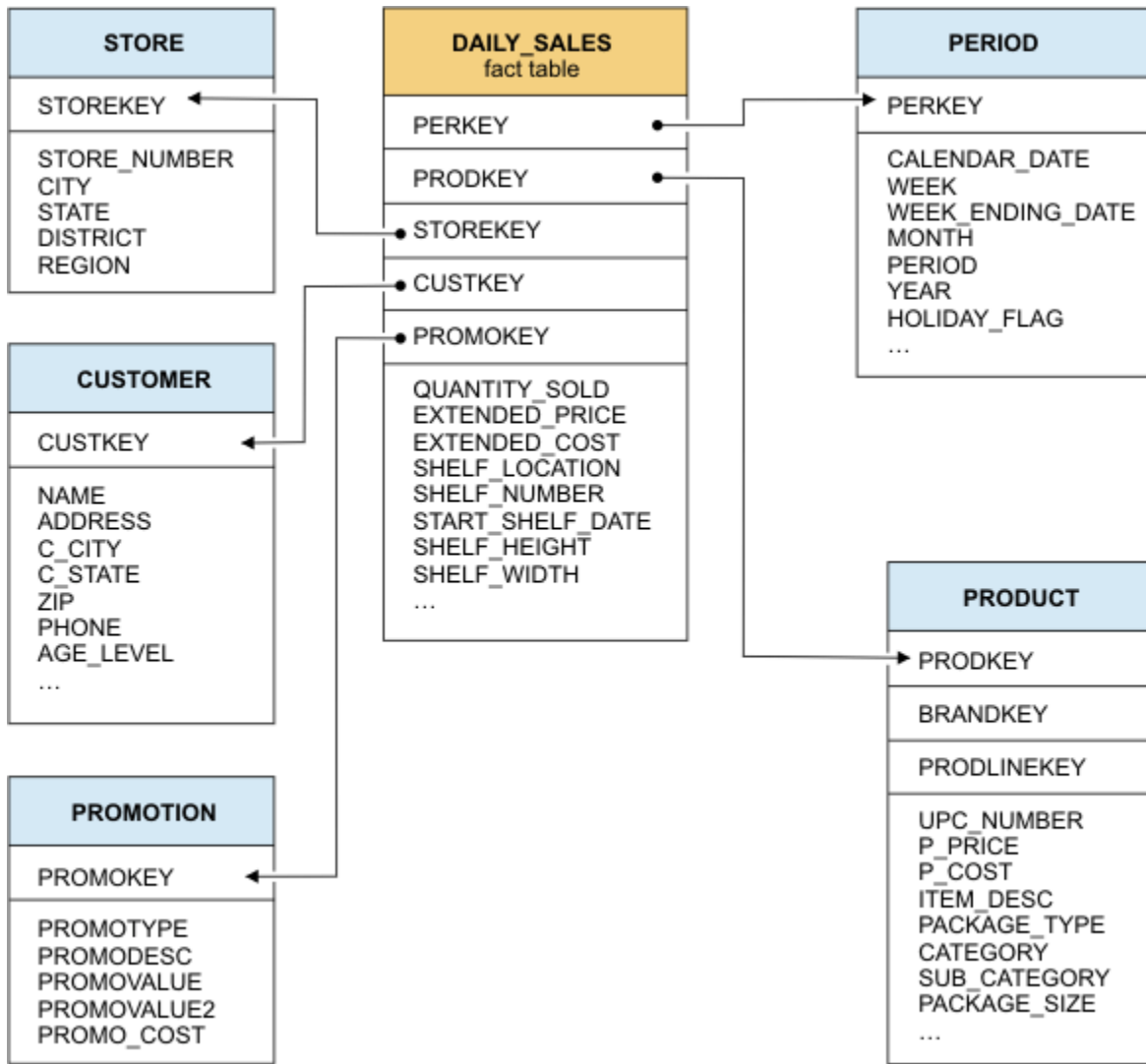
Figure 2. A data mart with the DAILY_SALES fact table
