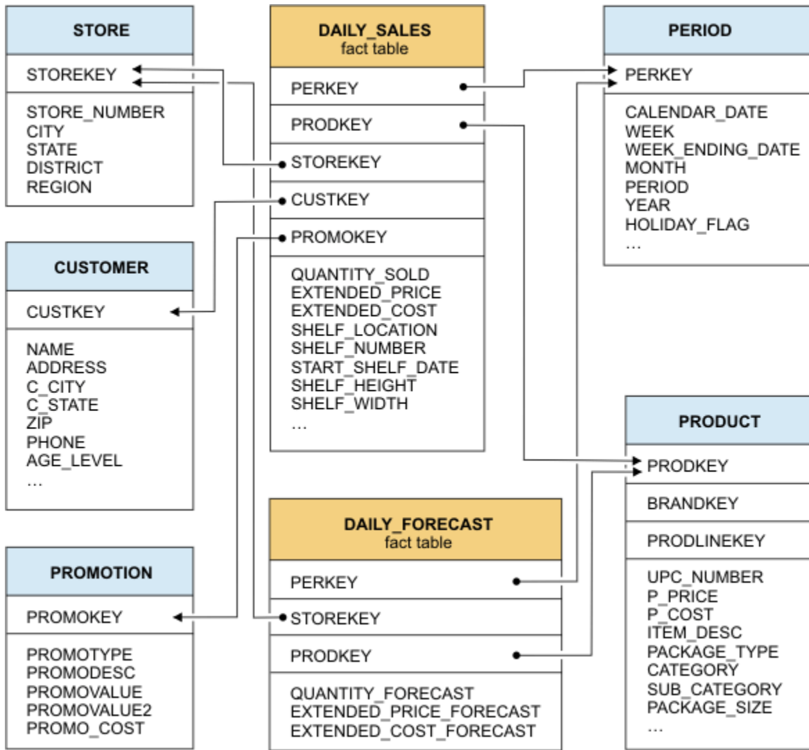
Figure 22. A sample star schema with two fact tables
