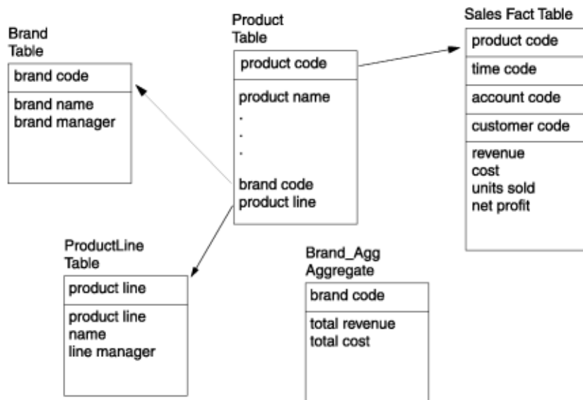
Figure 12. An example of a snowflake schema
