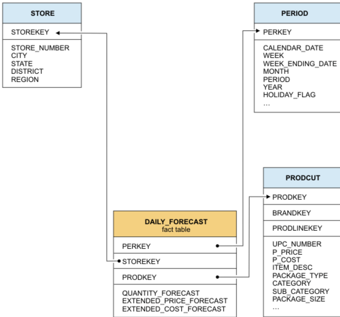
Figure 21. A data mart with the DAILY_FORECAST fact table
