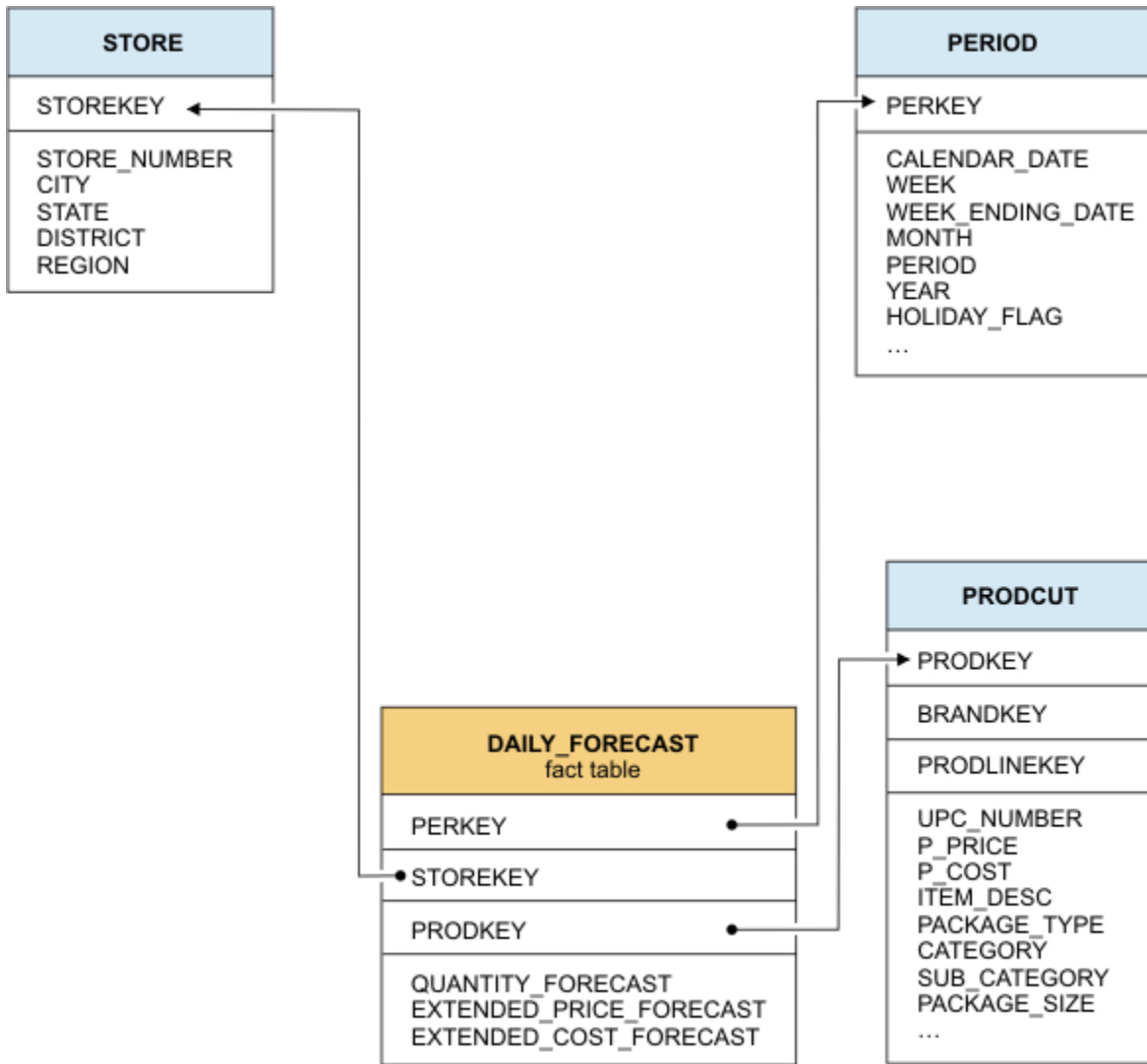
Figure 24. A data mart with the DAILY_FORECAST fact table
