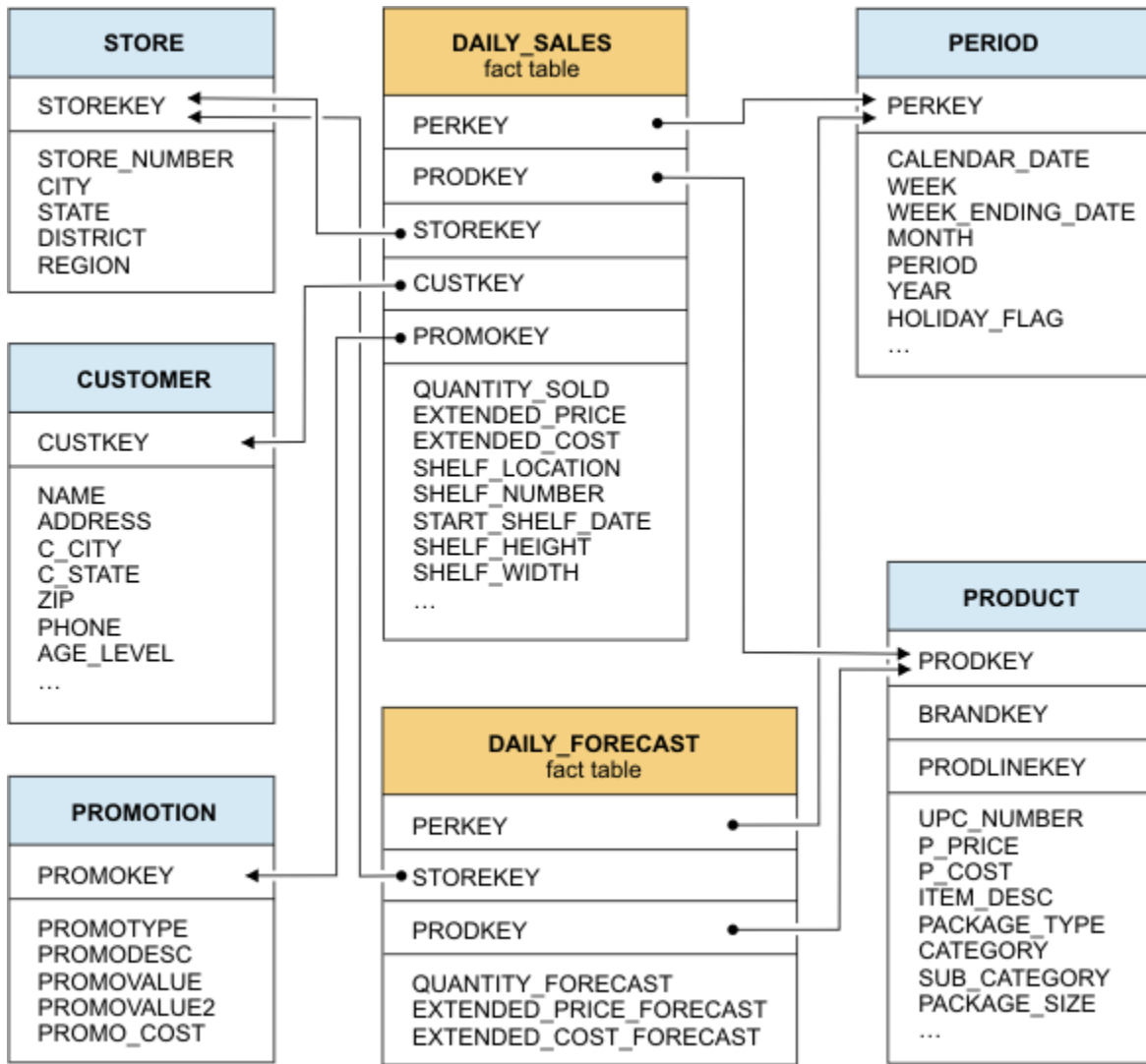
Figure 19. A sample star schema with two fact tables
