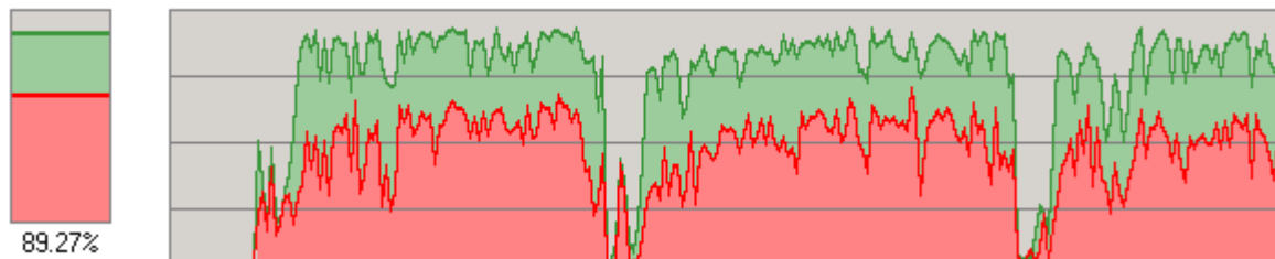
CPU Usage
